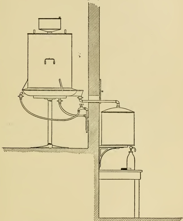
An arrangement of cooler and hand bottle filler. (Bureau of Animal Industry, Bull. 104.)
